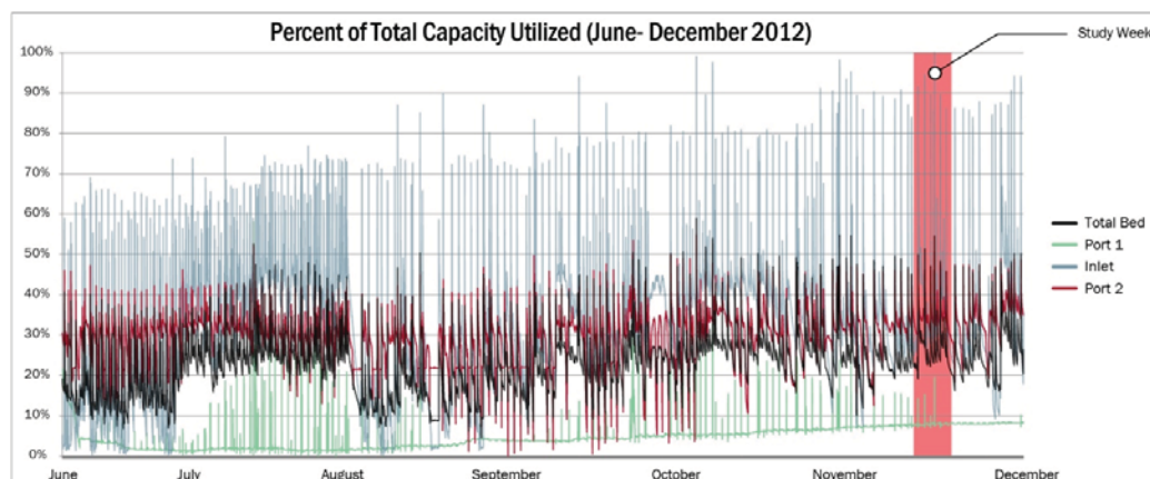
Figure 5: Saturation values within greywater bed during first six months of study. The area highlighted in red indicates the study week shown in Figure 6.
