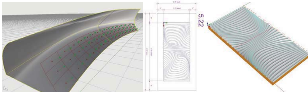
Figure 12: Left: Developable surface constrained by face normal angles, modeled in Rhinoceros; Middle: tool paths exported for use by RhinoCam; Right: Simulation of panel surface stock for CNC routing. Source: (Author 2013)
