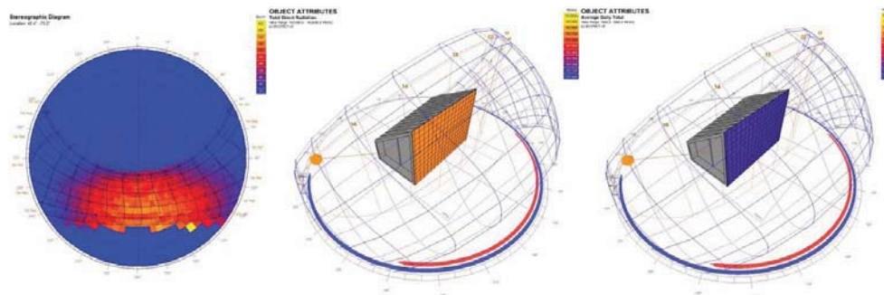
Figure 10: Left: total monthly stress south-facing façade (sun-path diagram); Middle: annual cumulative incident solar radiation (direct only); Right: annual cumulative photosynthetically active radiation (direct only). Source: (Author 2013).
