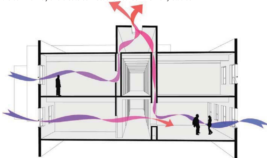
Figure 6: Renovated half walls to facilitate cross ventilation. Stack ventilation occurs through existing ductwork.
